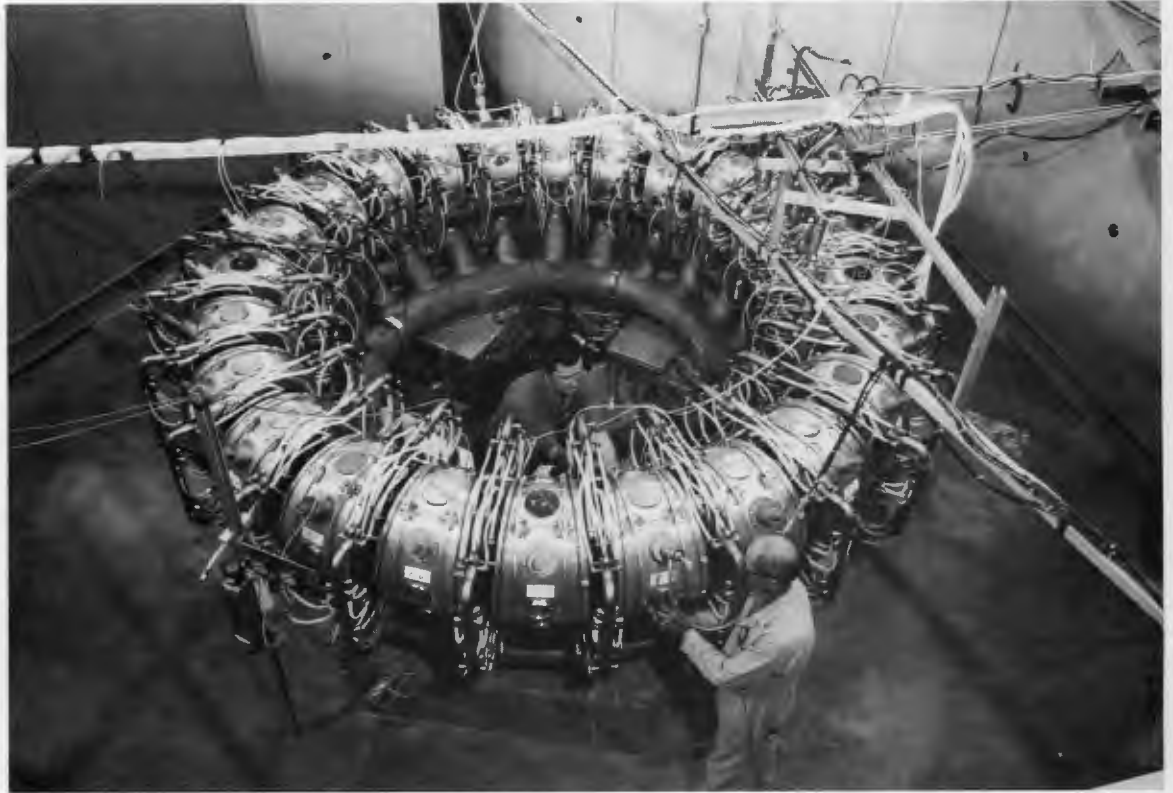
ELMO Bumpy Torus, built at ORNL for fusion energy experiments, set a record for plasma heating.
