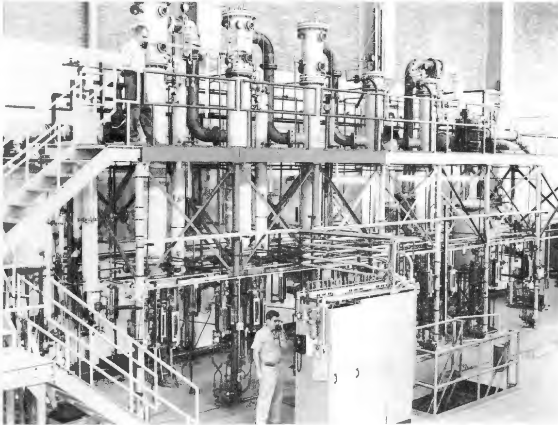
ORNL's desalination pilot plant used highly efficient heat transfer tubes to desalt large amounts of seawater.
