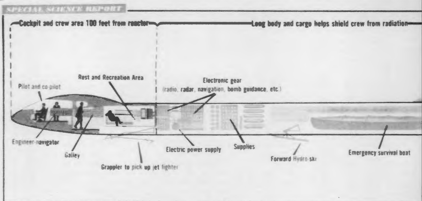
Diagram of a proposed nuclear aircraft, published in Newsweek in the 1950s.
