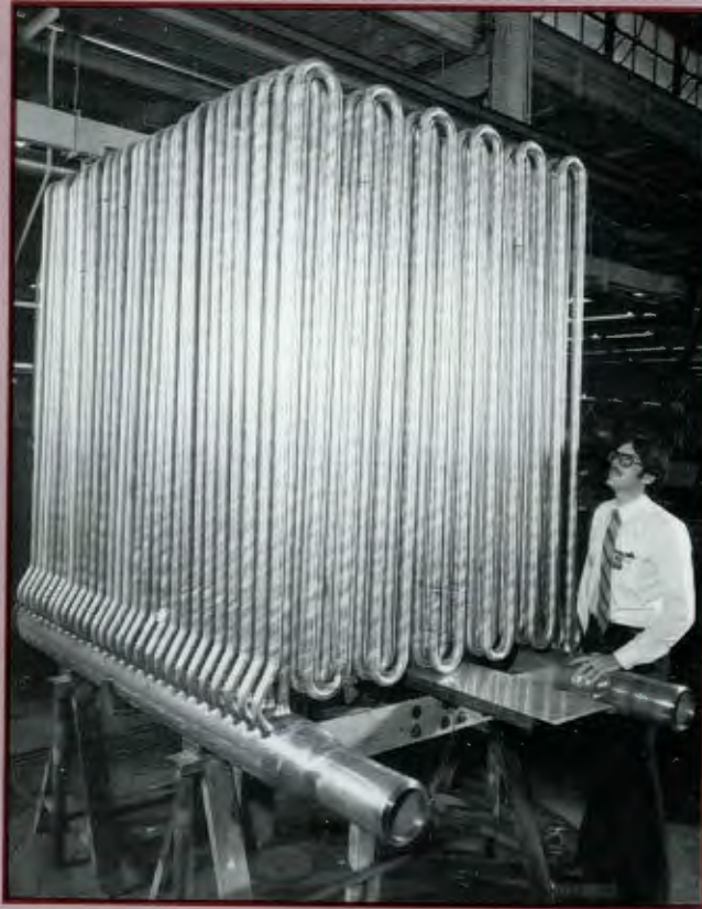
Tom Conley inspects a heat exchanger later installed in the Component Flow Test Loop, a key experimental facility for DOE's High Temperature Gas-Cooled Reactor Program.
