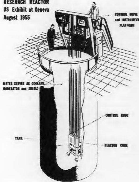
Drawing of "swimming pool" reactor designed and built for display at the 1955 Geneva Conference.
