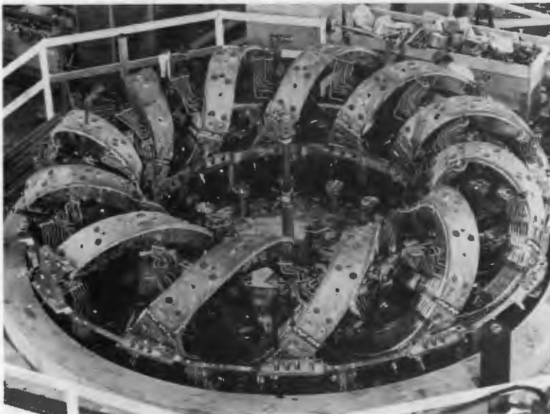
The coils of the Advanced Toroidal Facility, an experimental fusion reactor, which was completed in 1987 and produced its first fusion plasma in 1988.
