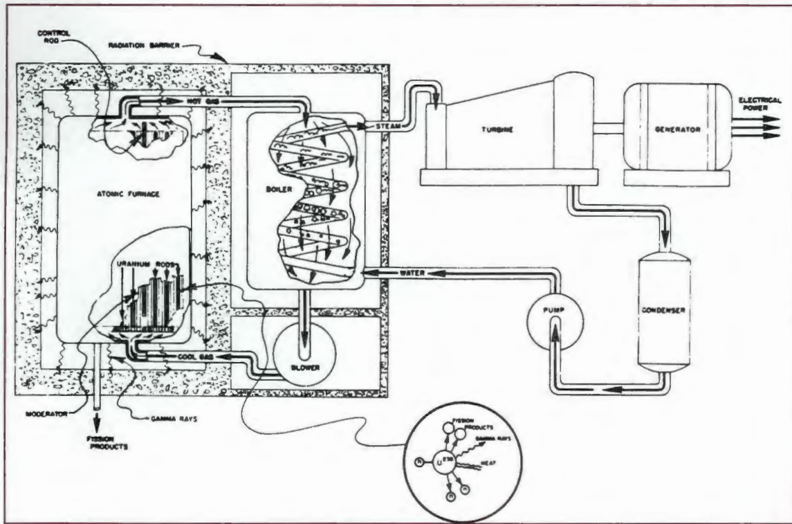
This 1946 sketch was the first released by the Laboratory to explain to the public the proposed use of a nuclear reactor to generate electricity.
