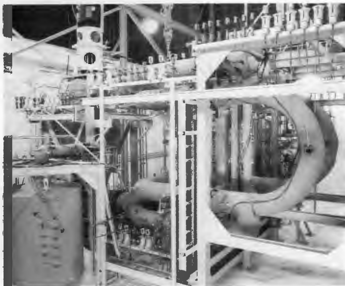
Equipment for the Molten Salt Reactor Experiment.
