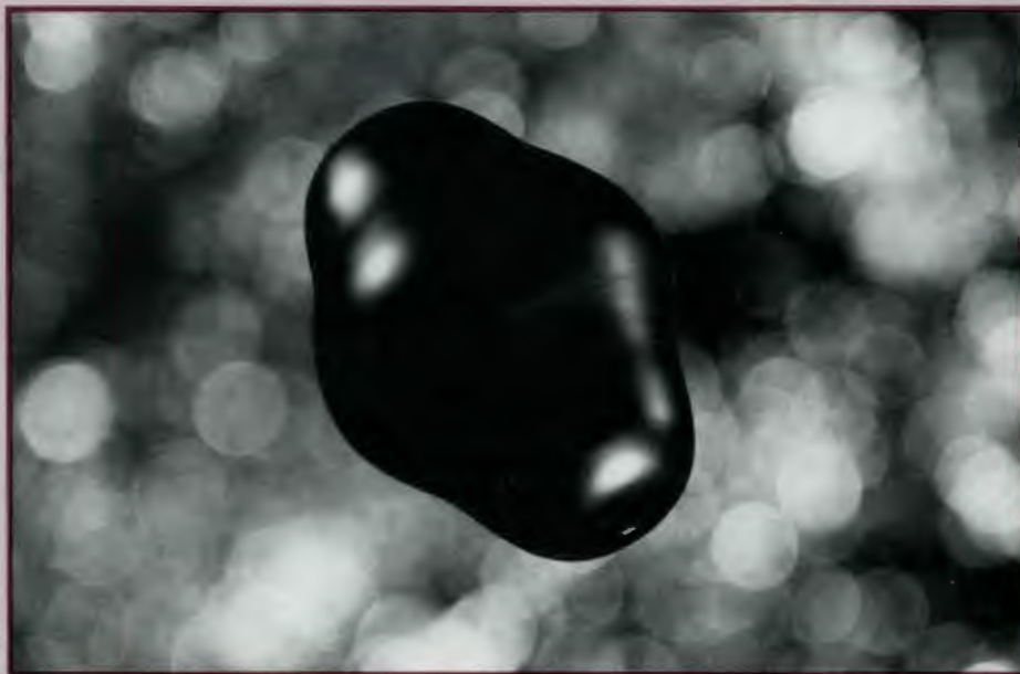
The likely shape of a deformed uranium-234 nucleus as determined by the results of 1971 accelerator studies.
