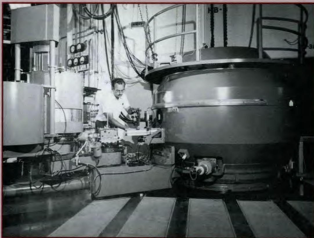
Bob Nicklow installs a remotely controlled diaphragm that limits the size of the neutron beam in experiments with the triple-axis spectrometer at a beam port of the High Flux Isotope Reactor.
