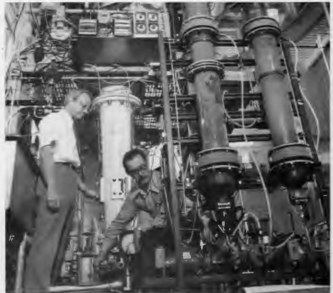
Charles Scott and Charles Hancher examine a fluidized-bed bioreactor used to reduce nitrate concentrations in wastewater.
