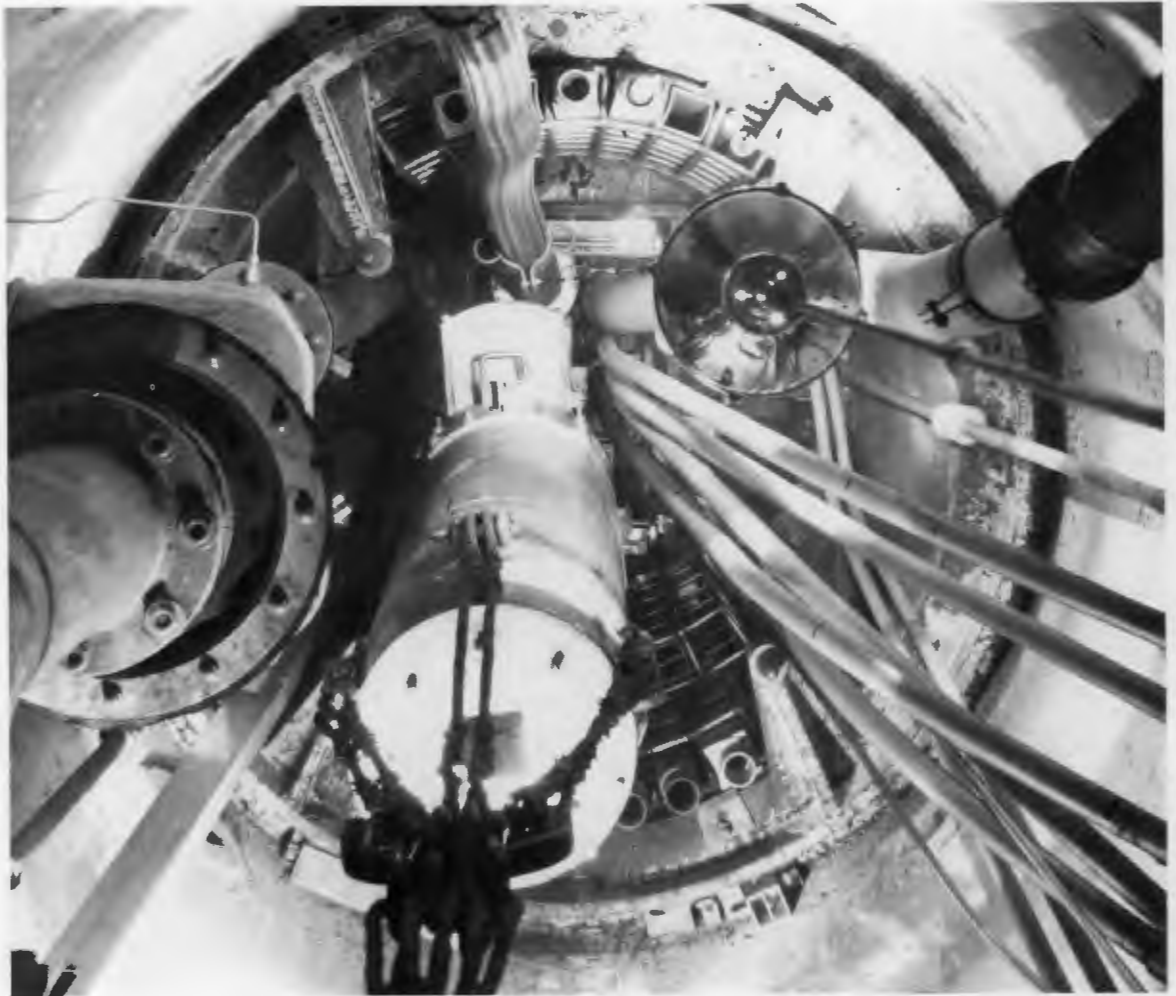
The core of the Low Intensity Test Reactor.
