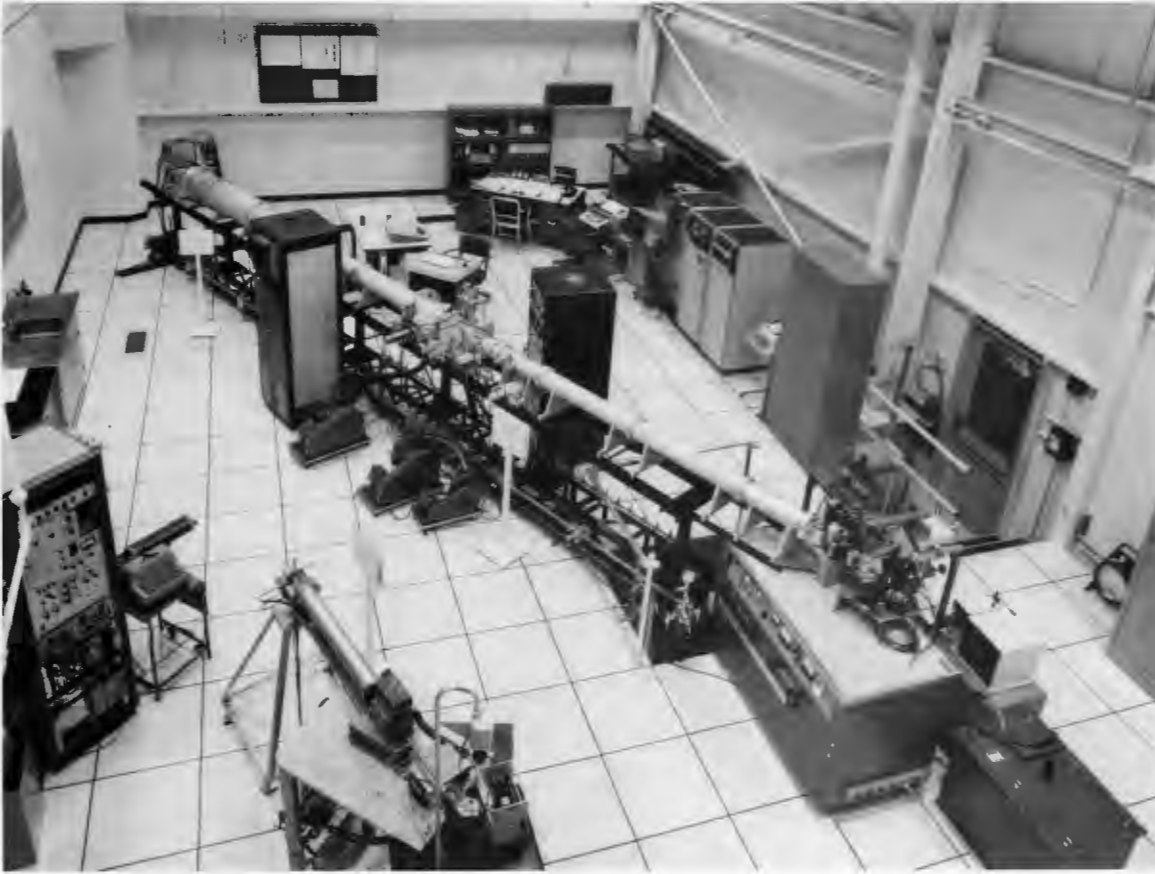
The small-angle X-ray scattering device developed by Robert Hendricks became part of the National Center for Small-Angle Scattering Research established in 1978.
