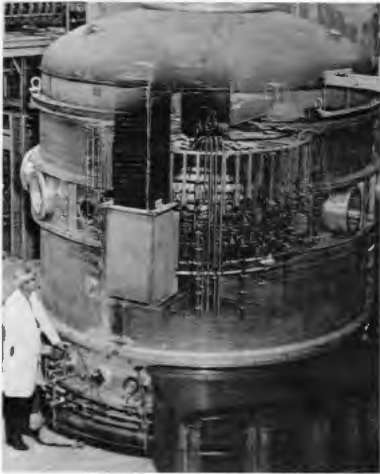
The Oak Ridge experimental tokamak, called ORMAK, used for fusion energy experiments.
