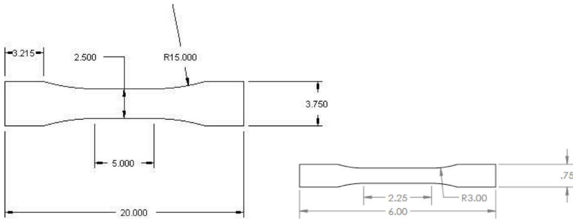
Figure 2. Test sample cut plan for BAAM dog bone tensile specimens (all dimensions in inches). The larger specimen (left) is 0.75" thick and the smaller sample (right) is 0.25" thick. Images are not to relative scale.
