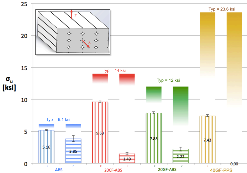
Figure 3. Tensile Strength of Techmer materials deposited on the BAAM system.
