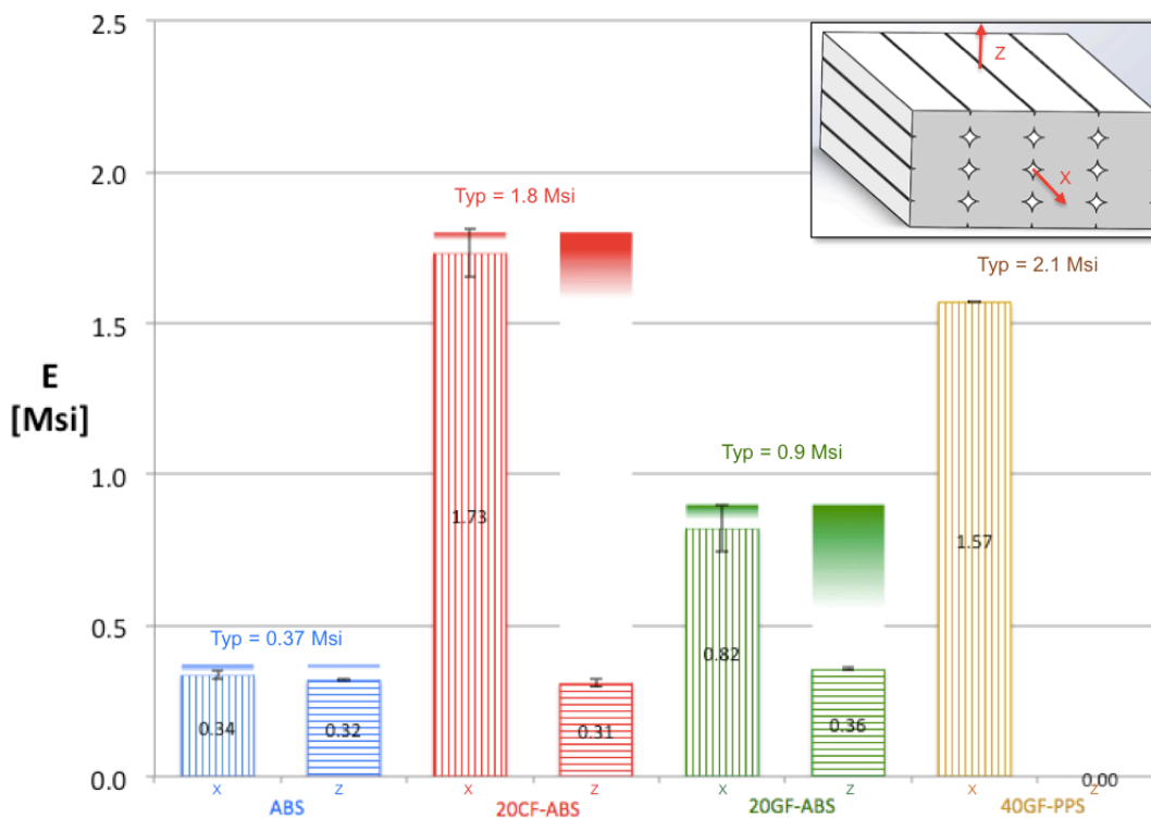
Figure 4. Tensile Stiffness of Techmer materials deposited on the BAAM system.
