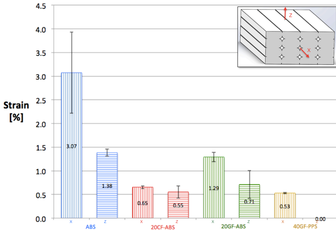
Figure 5. Tensile Elongation of Techmer materials deposited on the BAAM system.
