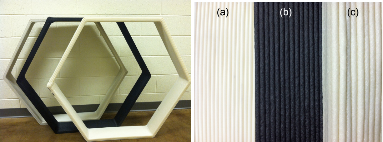
Figure 1. Hexagons (left) printed on BAAM system for mechanical testing. Close-up of deposited walls (right) for (a) neat ABS, (b) CF-ABS, (c) GF-ABS
